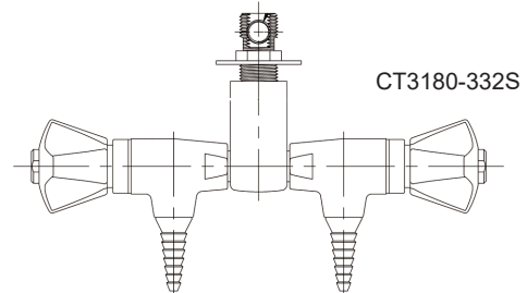
Double, Needle Valve - ColorTech Knobs
