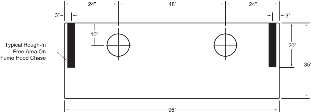
SERVICE ROUGH-IN DETAIL (FOR 96" & 120" HOODS)
